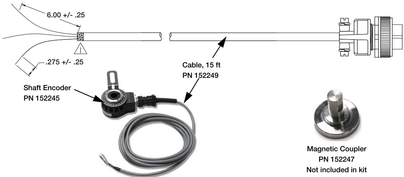
Figure 1-1. Shaft Encoder Kit (PN 152626)
