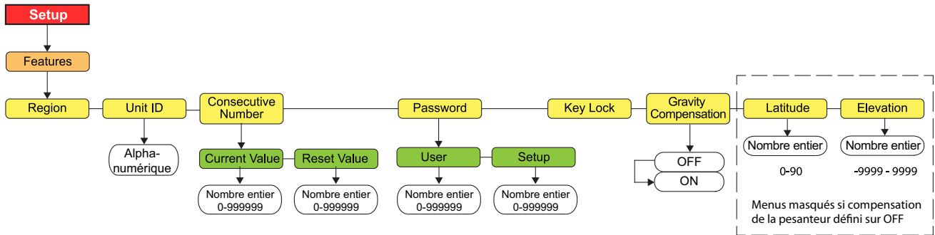
Figure 3-11. Menu Features
