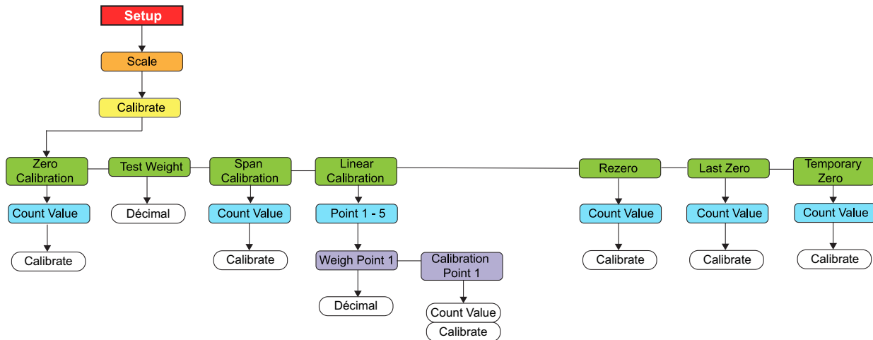
Figure 4-1. Menu Calibration
