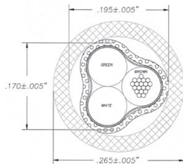
Three-conductor cable
