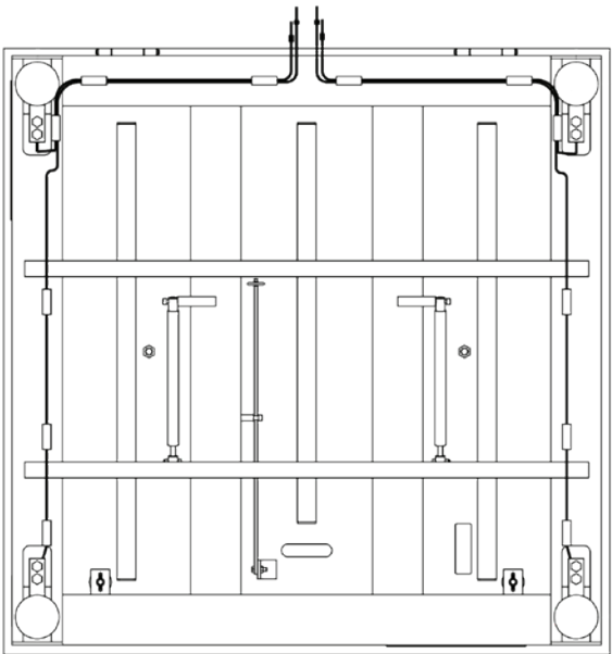
Underdeck View
