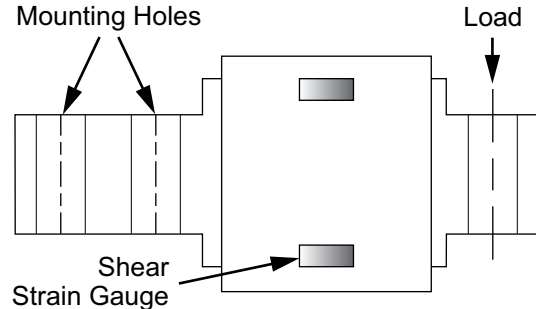
Figure 1-4. Cantilever Beam
