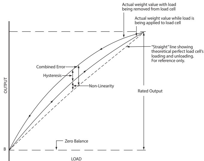
Figure 6-1. Calibration Curve
