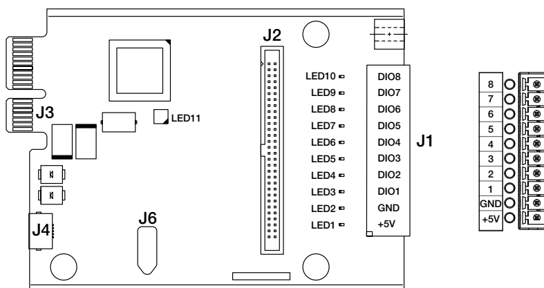
Figure 2. DIO Option Card
