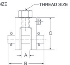
Clevis Mount with pin
