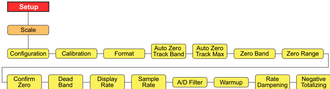
Figura 4-5. Setup – Menú Scale
