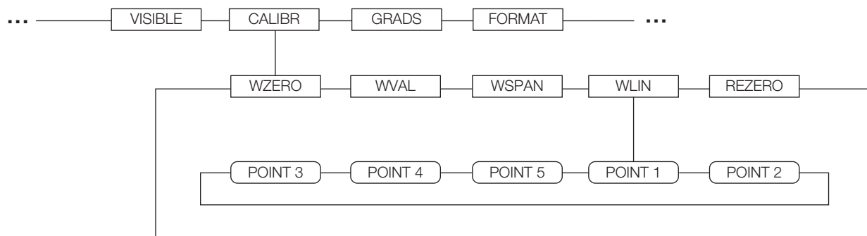
Figura 4-1. Submenú Calibration (CALIBR)
