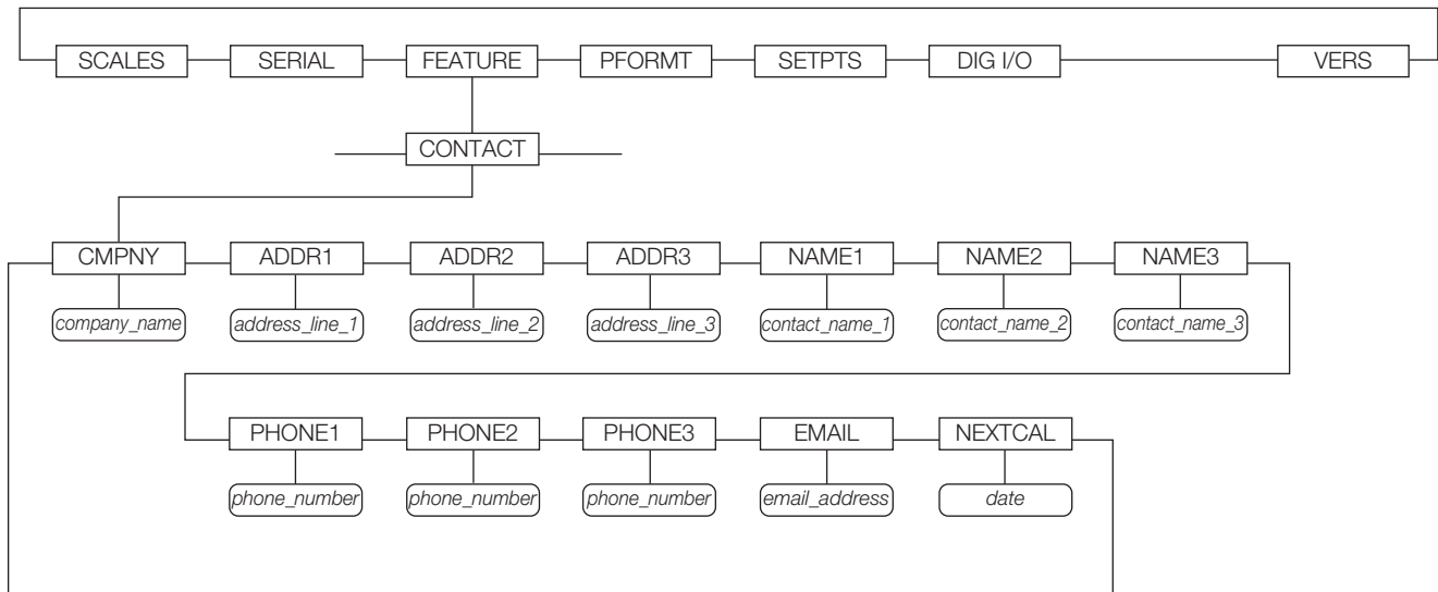
Figura 3-14. Submenú CONTACT
