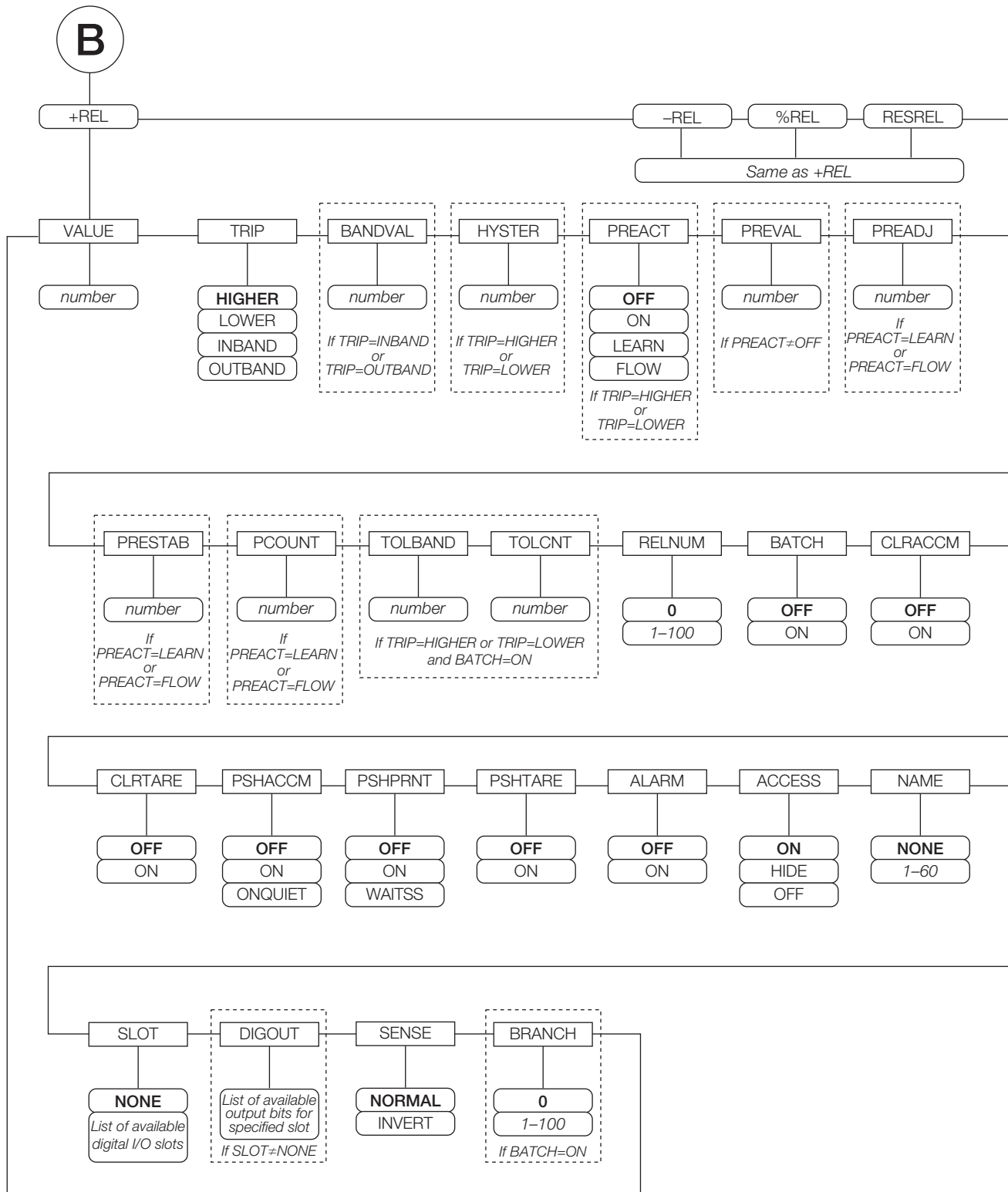
Figura 9-3. Parámetros de Setpoints +REL, -REL, %RELS y RESREL
