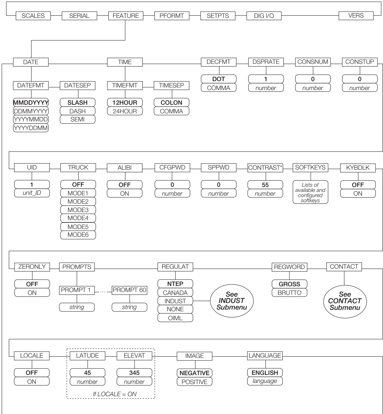
Figura 3-13. Menú FEATURE
