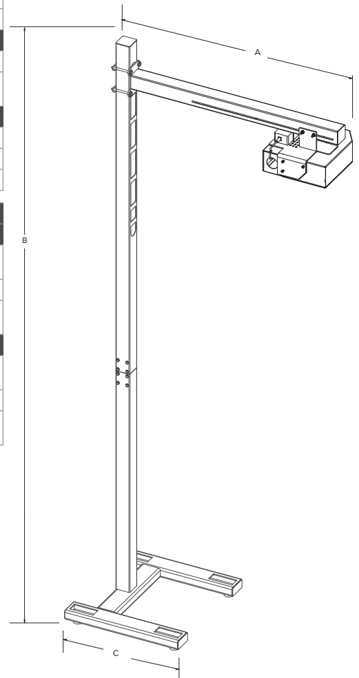
Optional iDimension Plus XL Floor Mount Stand Assembly Dimensions
