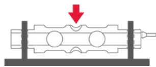
A double-ended beam load cell is secured at both ends with the load applied to the center.
