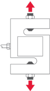
S-beam load cells are used to suspend a weighing vessel with tension applied through stretching.
