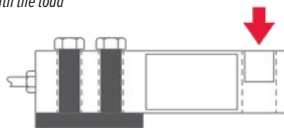
A single-ended beam load cell is secured at one end with the load applied to the opposite end.
