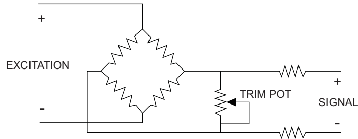
Figure 24-2. Signal Trimming Procedure
