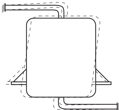
Figure 15-5. Weigh Vessel with Rigidly-Attached Piping
