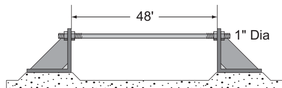
Figure 15-2. Stay Rod
