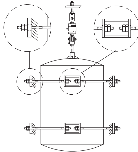
Figure 20-2. Stay Rod Application
