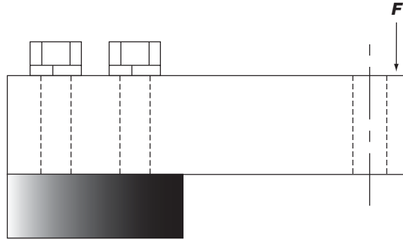
Figure 4-3. Eccentric Loading
