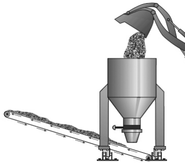
Figure 12-5. Loader Fed Weigh Hopper
