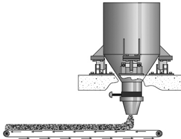
Figure 12-10. Loss in Weight System
