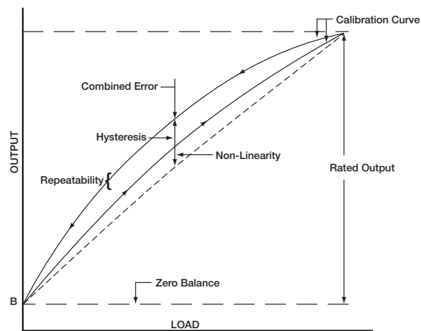
Figure 6-1. Calibration Curve
