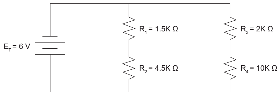
Figure 5-8. Parallel Circuit
