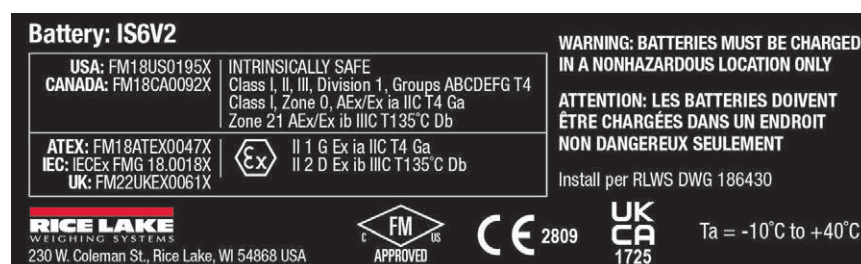
Figure 2. IS6V2 Battery Box Label
