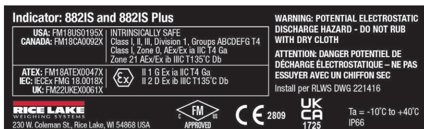
Figure 1. 882IS and 882IS Plus Indicator Label
